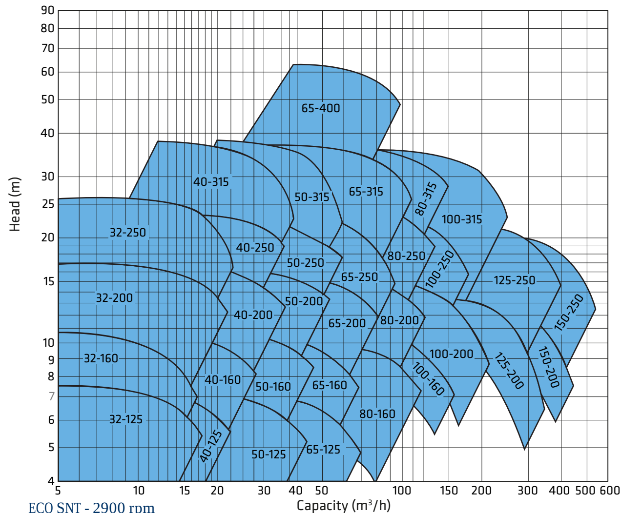
ECO SNT - 2900 rpm
