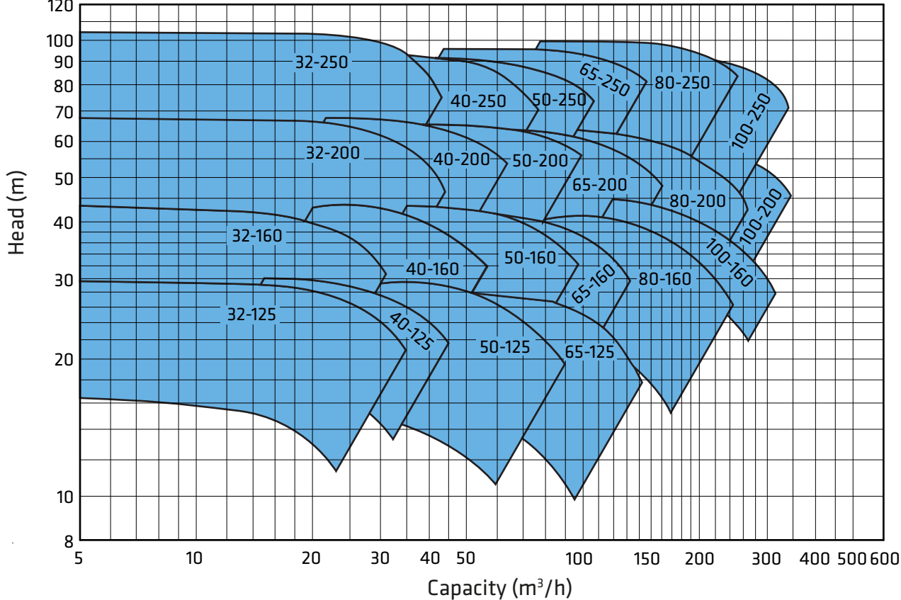
ECO SNT - 2900 rpm
